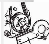
Crankshaft Locking Tool (Q)
