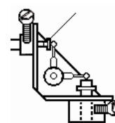
Pump Timing Components for Lucas, CAV Rotodiesel DPC Rotary Injection Pumps
