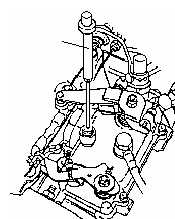
Pump Timing Components for Lucas, CAV Rotodiesel DPC Rotary Injection Pumps
