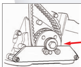
Crankshaft locking Tool
